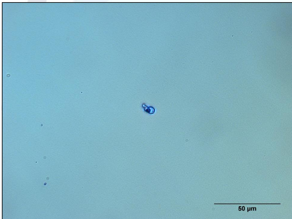
Fig. 4 Typical front surface damage morphology (Energy density 13.54 \text{ J/cm}^2 , damage after 24 pulses)
