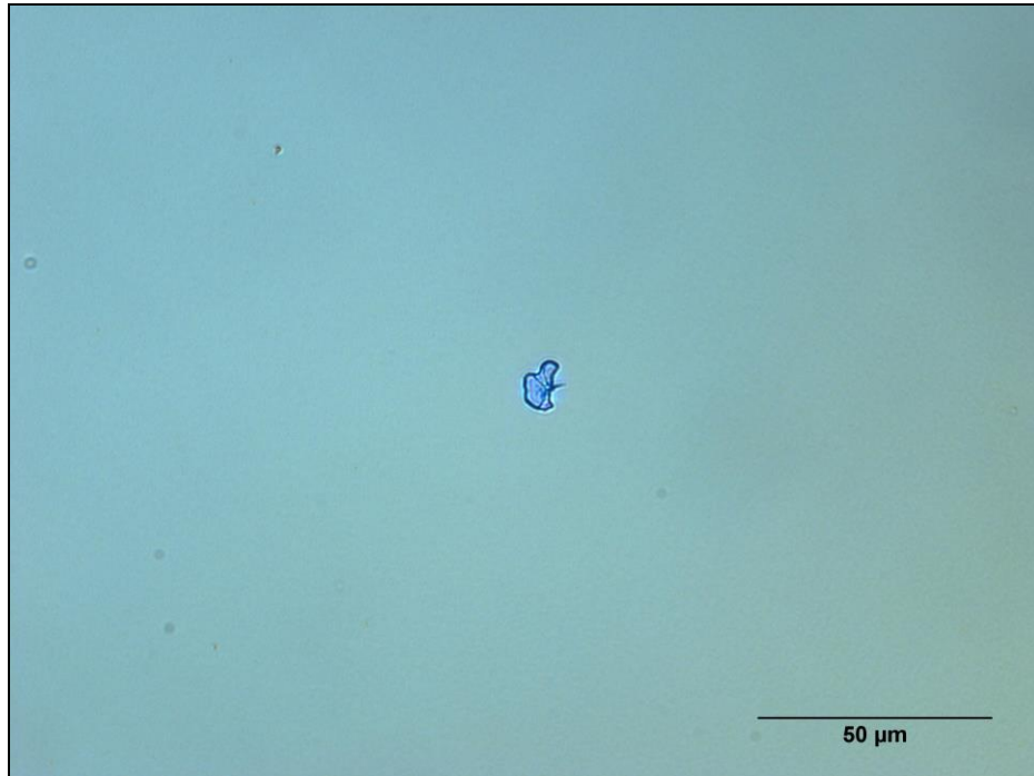
Fig. 3 Typical front surface damage morphology (Energy density 33.07 \text{ J/cm}^2 , damage after 1 pulse)
