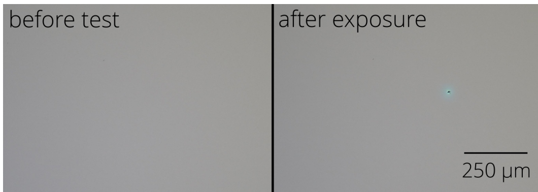
Figure 5. Typical damage morphology: fluence 11.9 J/cm 2 , damage after 202 pulse(s).
