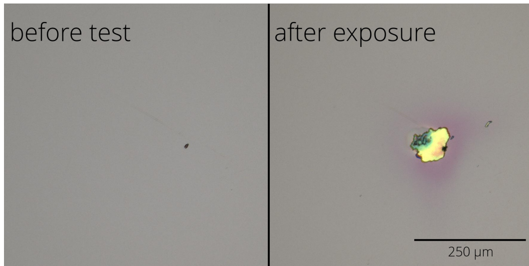
Figure 4. Typical damage morphology: fluence 23.1 \text{ J/cm}^2 , damage after 153 pulse(s).
