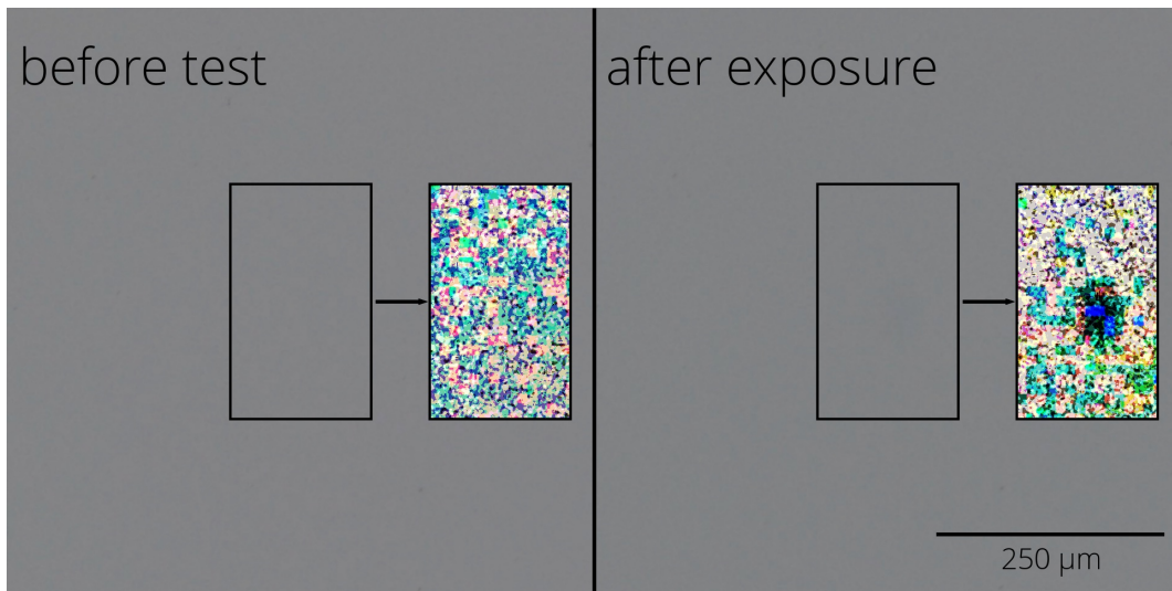
Figure 5. Typical damage morphology: fluence 38.0 J/cm 2 , damage after 1000 pulse(s). High contrast image.
