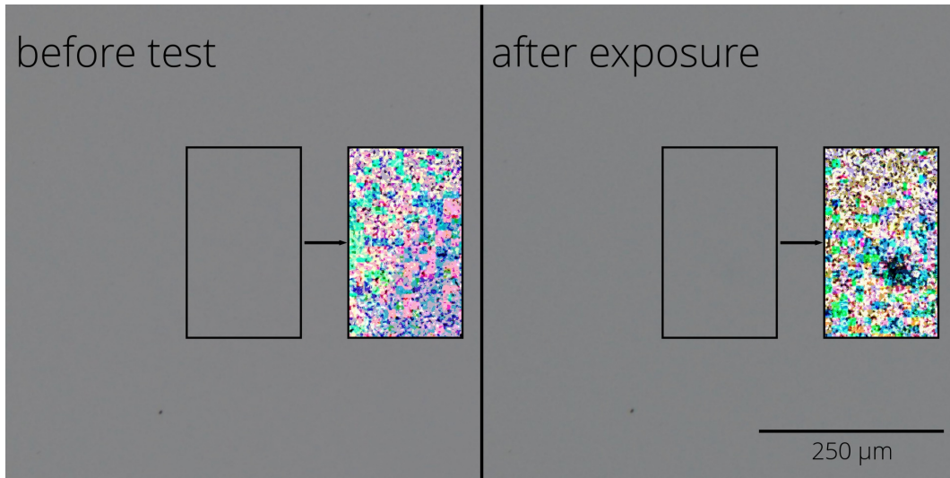
Figure 4. Typical damage morphology: fluence 13.2 J/cm 2 , damage after 1 pulse(s). High contrast image.
