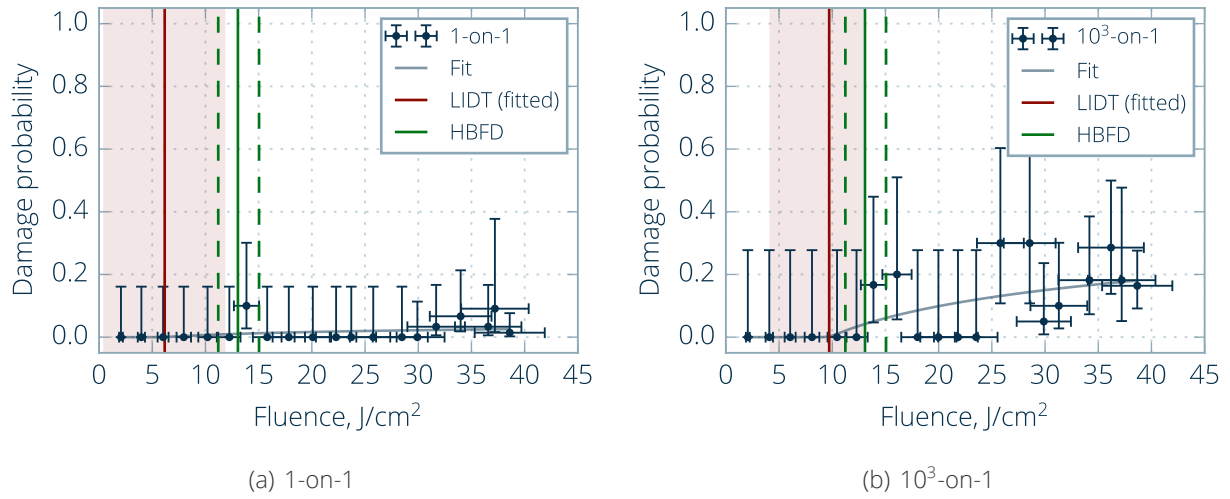
Figure 3. Damage probability plots. 4
